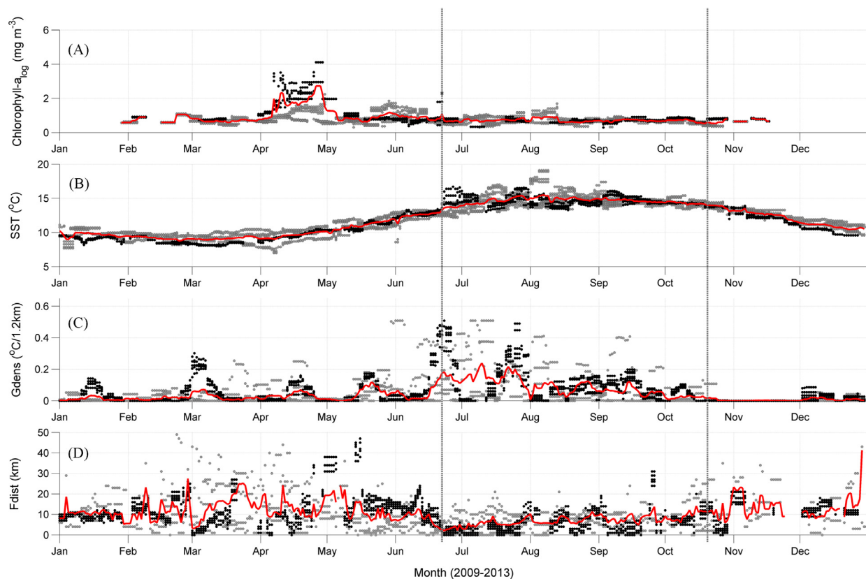
Fig. 2. Bio-physical oceanographic conditions observed at each the deployment stations over the five years (plotted in light grey with those from the year 2010 highlighted in black). Daily averages (across sites/year) are shown in red. From top to bottom: (A) log surface chlorophyll-a LogChlorophyll , (B) sea surface temperature SST , (C) front gradient Gdens and (D) distance to closest front Fdist . Seasonal fluctuations in the bio-physical conditions experienced across the site are noted. Warmer temperatures and increased frontal activity correspond to the summer months of June to October (the extents of which are indicated by the vertical dashed lines). A peak in surface chlorophyll-a in late April indicates the occurrence of the annual spring bloom. (For interpretation of the references to colour in this figure legend, the reader is referred to the web version of this article.)
