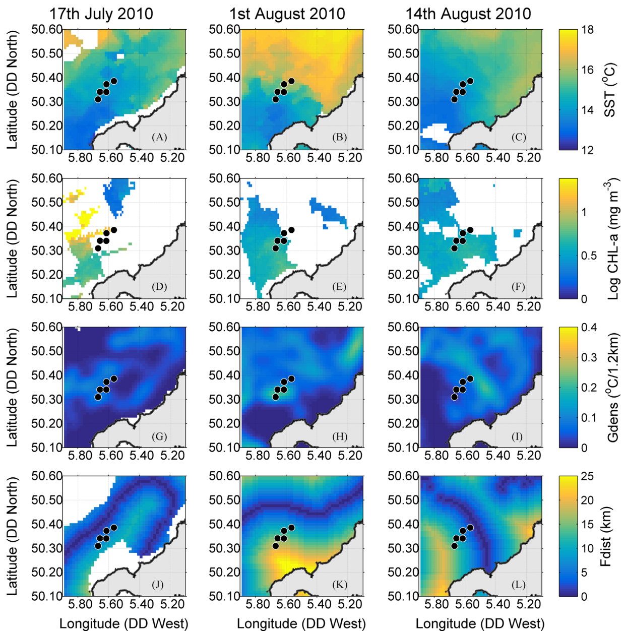
Fig. 4. Bio-physical conditions experienced across the site during the summer of 2010. From top to bottom: sea surface temperature (SST) (A:C), log surface chlorophyll-a ( LogChlorophyll ) (D:F), front gradient Gdens (G:I) and distance to closest front ( Fdist ) (J:L). The locations of deployment stations are marked by black dots with white outlines. Each column corresponds to a different date as indicated: 17th July (A, D, G & J), 1st August (B, E, H & K) and 14th August (C, F, I & L). A cycle of SST warming (approximate for thermal stratification) and cooling (approximate for water mixing) is noted across the deployment stations between dates, which coincides with variation in the position and intensity of the front.
